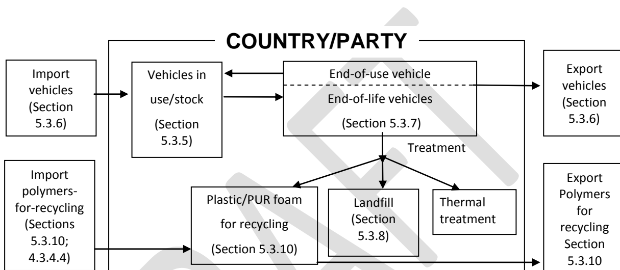
Figure 5-1: Material flow of the transport sector and the life cycle stage for POP-PBDEs inventories (Note: countries with production need to consider manufactured vehicles)
